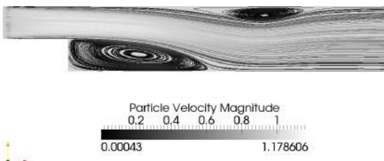
Figure 1: Velocity magnitude of the dispersed phase for breakage case with 6000 nodes mesh and tolerance of 1 \times 10^{-6} at 0.3 seconds.
