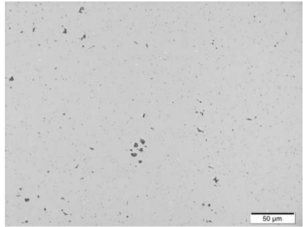
Figure 3: Optical microscopy image of SiC sample with 500x magnification after sanding and polishing at a depth of 200 \mu m.
