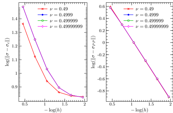
Figure 2: Convergence study for \boldsymbol{\sigma} in H(\text{div}) norm of SHDG approximations with discontinuous multiplier, \beta_0 = 2 , \beta_n = 7 , \delta_1 = 40 and \delta_2 = -1/2 .
